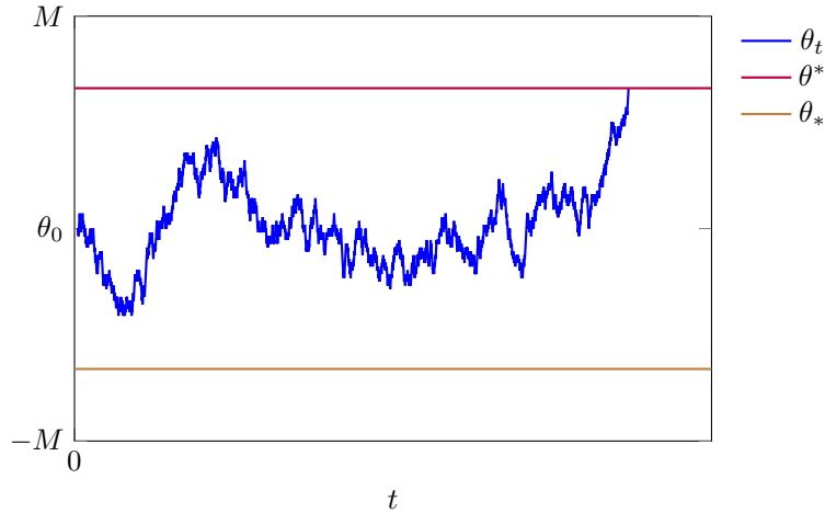
Figure 2: Sample equilibrium path where player 2 wins
