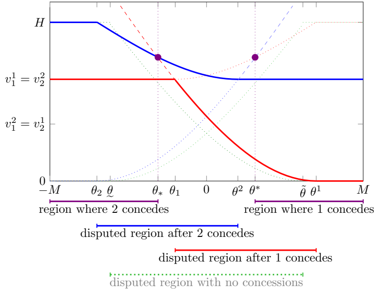
Figure 6: Concessions under moderately heterogeneous valuations
