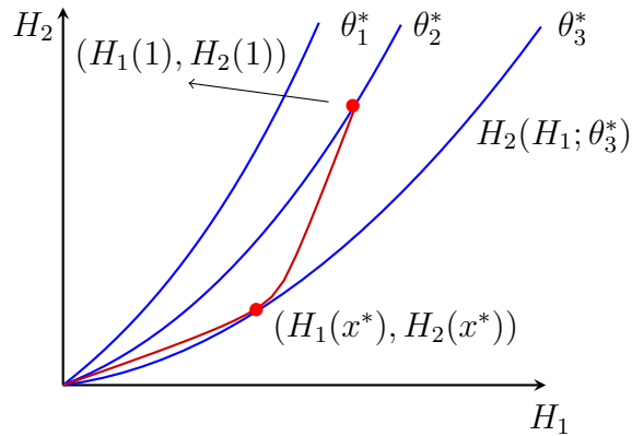
Figure 4: Level curves, feasible prize pairs, and optimal concession x^*
