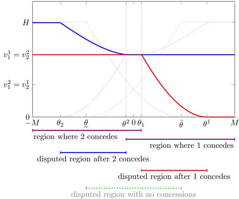
Figure 5: Concessions under highly heterogeneous valuations
