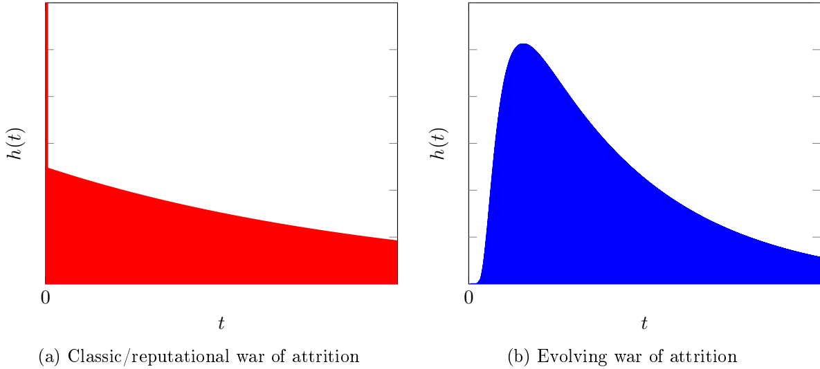
Figure 3: Density of length of the war
